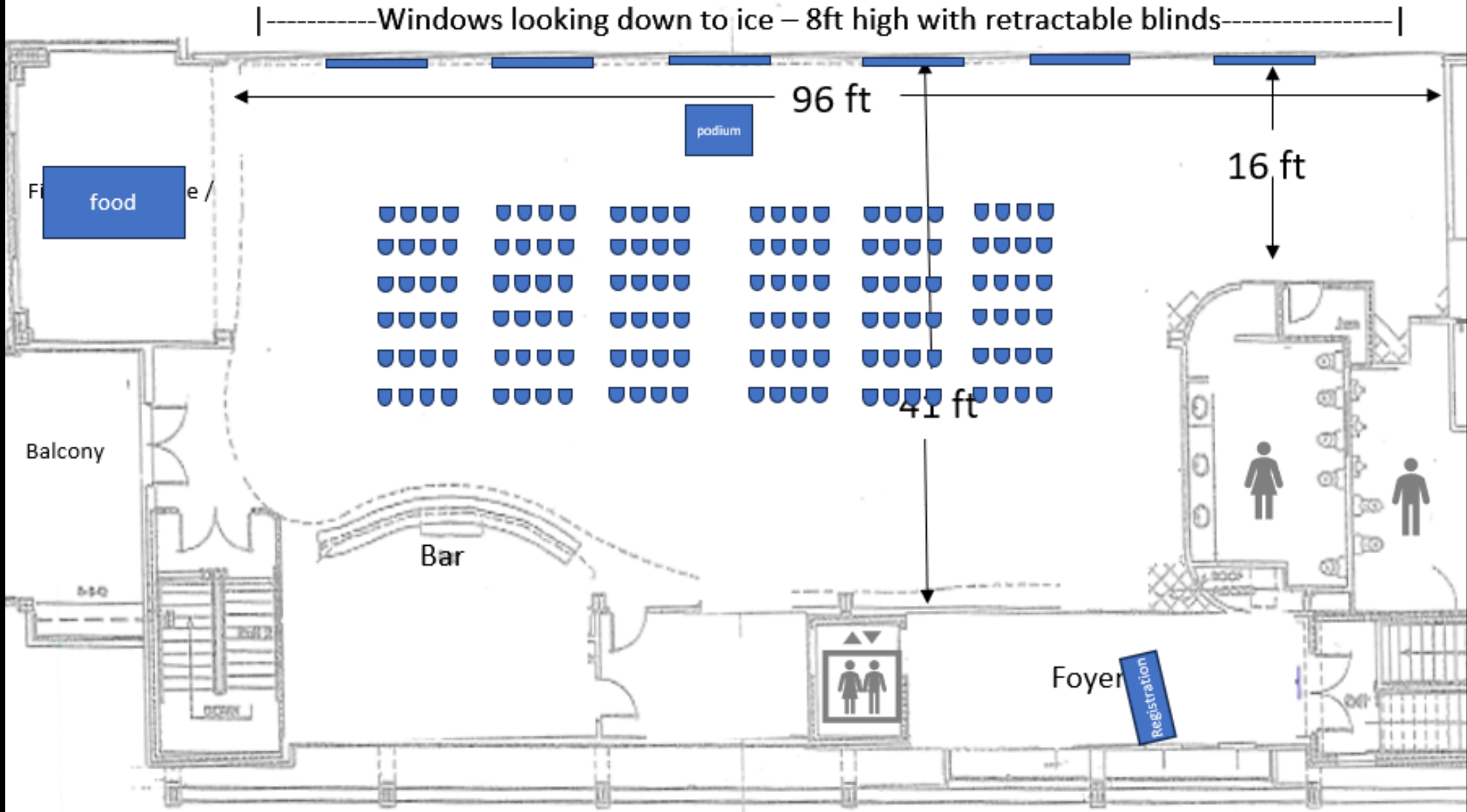
Floor Plan - Upstairs
